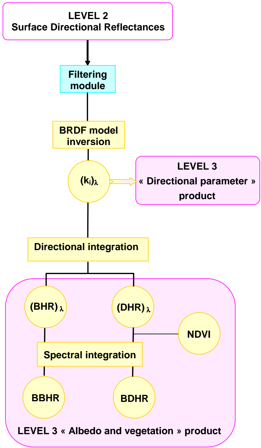
Figure 2 : Outline of the Level 3 Land Surface processing line
